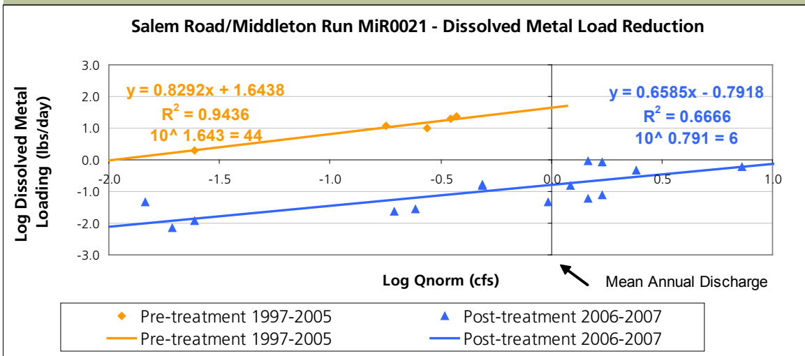
Figure 5. Dissolved Metal Load Reduction
