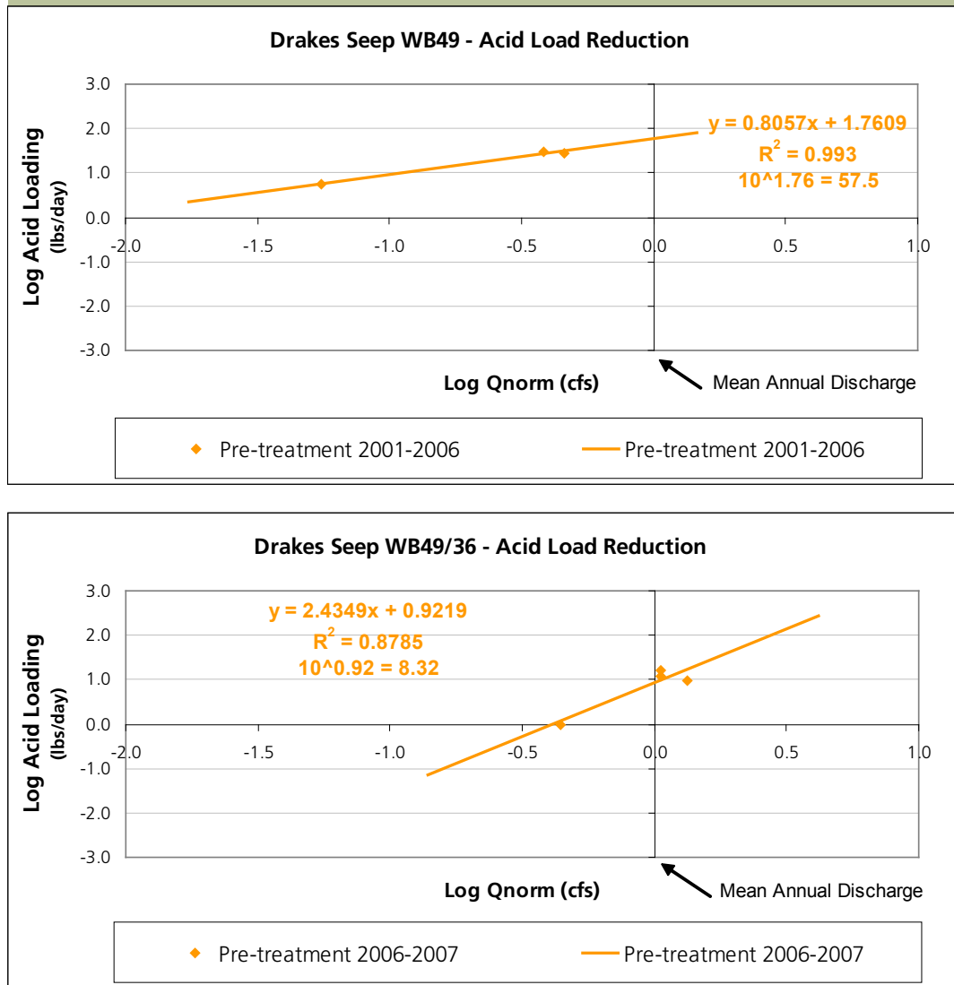
Fig. 1 Pre-construction acid loads
