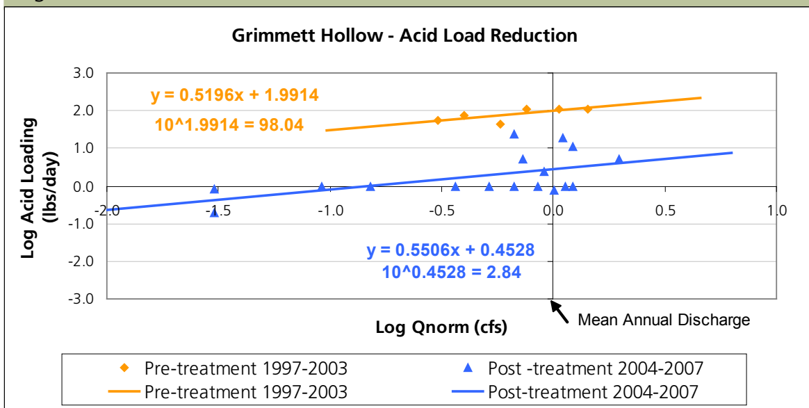
Figure 3. Acid Load Reduction
