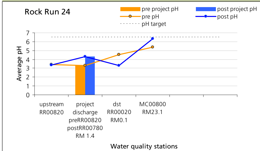
Figure 1. Pre and Post pH
