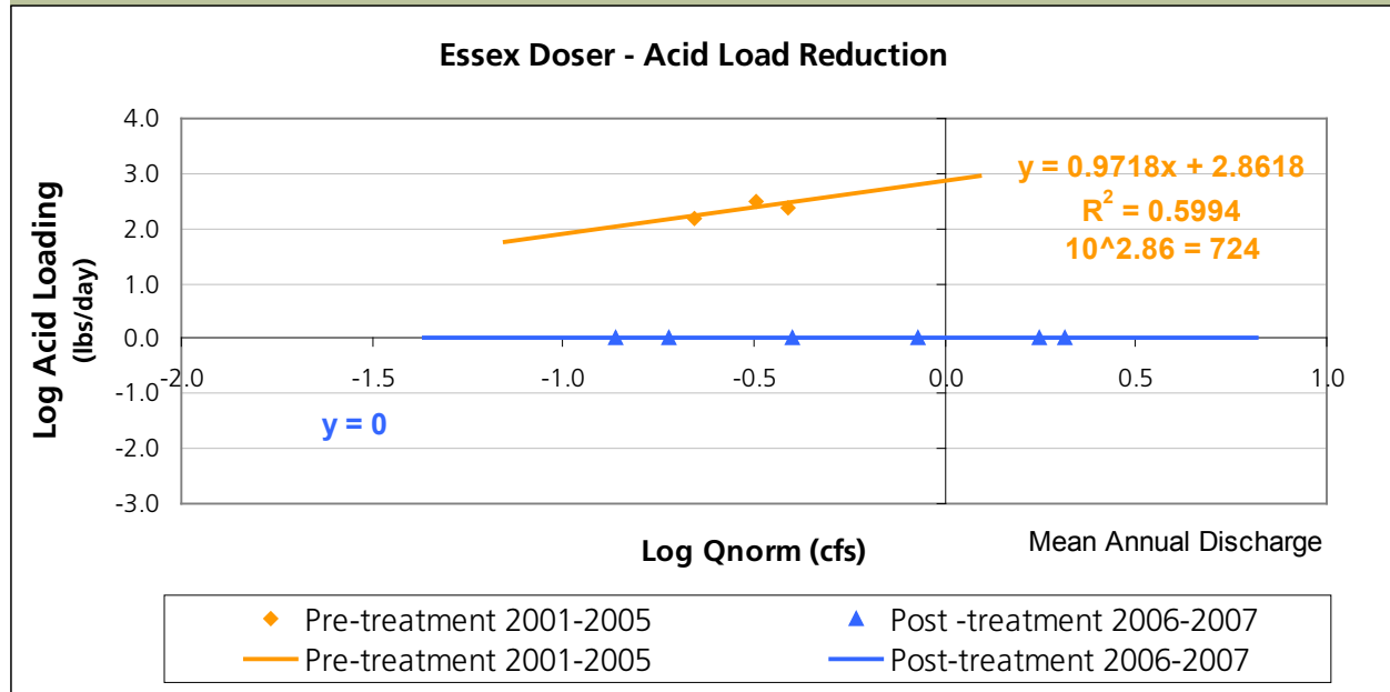
Figure 3. Acid Load Reduction
