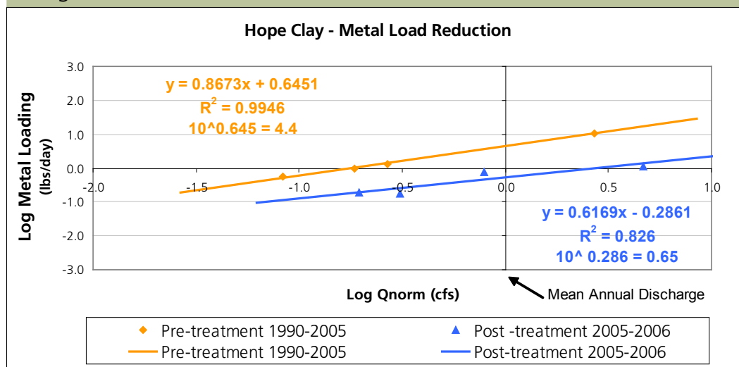
Figure 4. Metal Load Reduction
