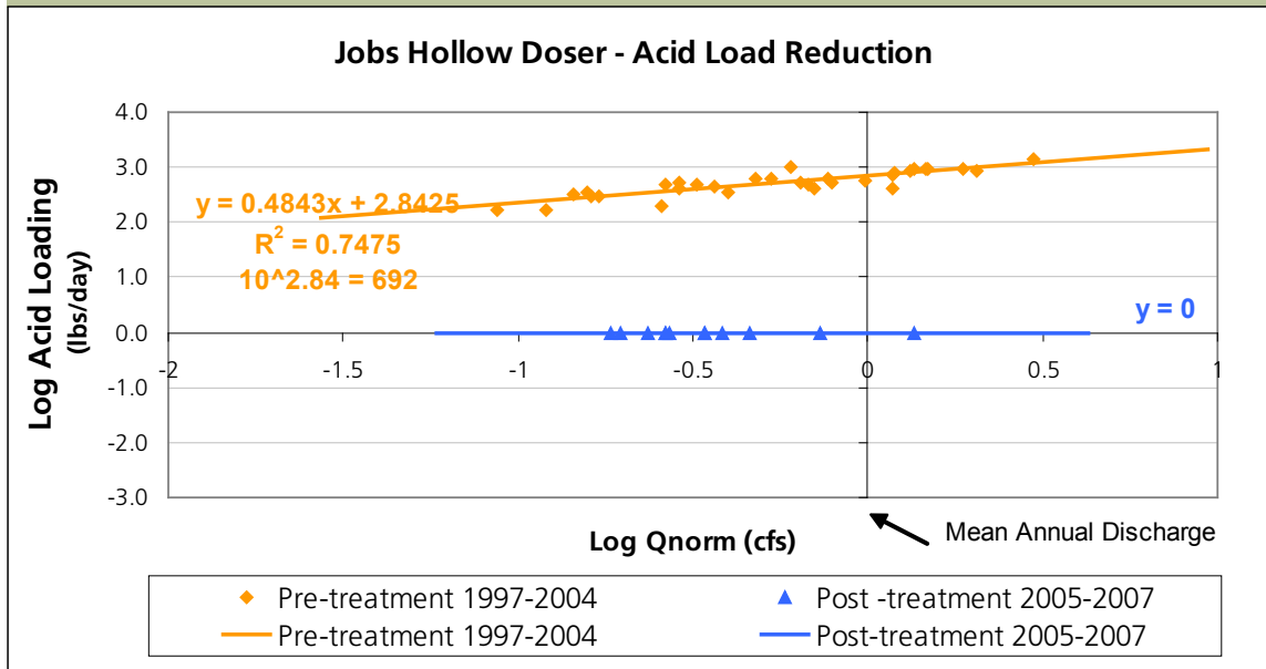
Figure 3. Acid Load Reduction
