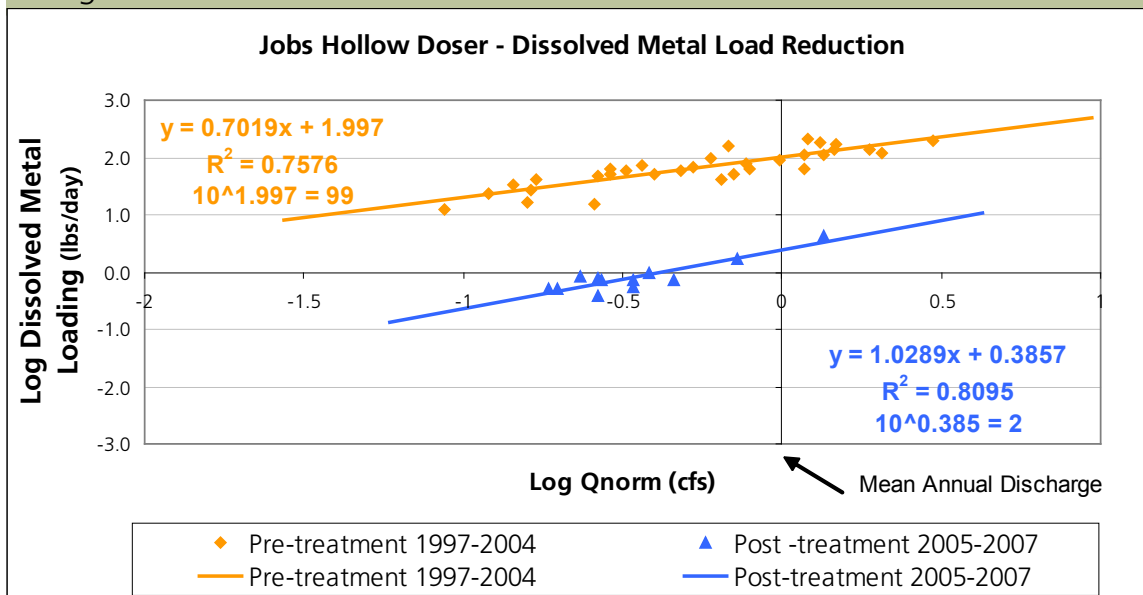
Figure 4. Metal Load Reduction
