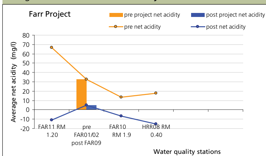
Figure 2. Pre and Post Acidity
