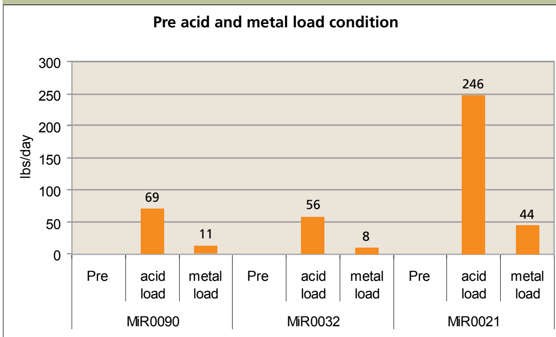
Figure 3. Acid Load Reduction Three project discharges at the Salem Road Project Site
