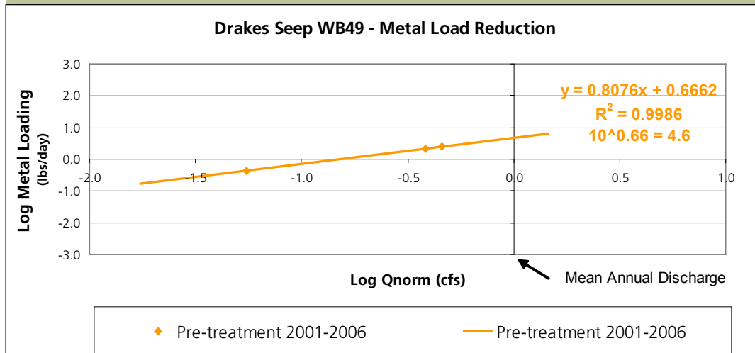
Fig. 2 Pre-construction metal loads
