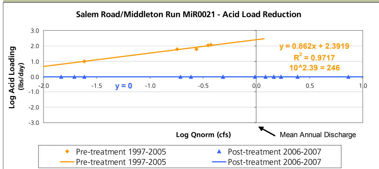
Figure 4. Acid Load Reduction
