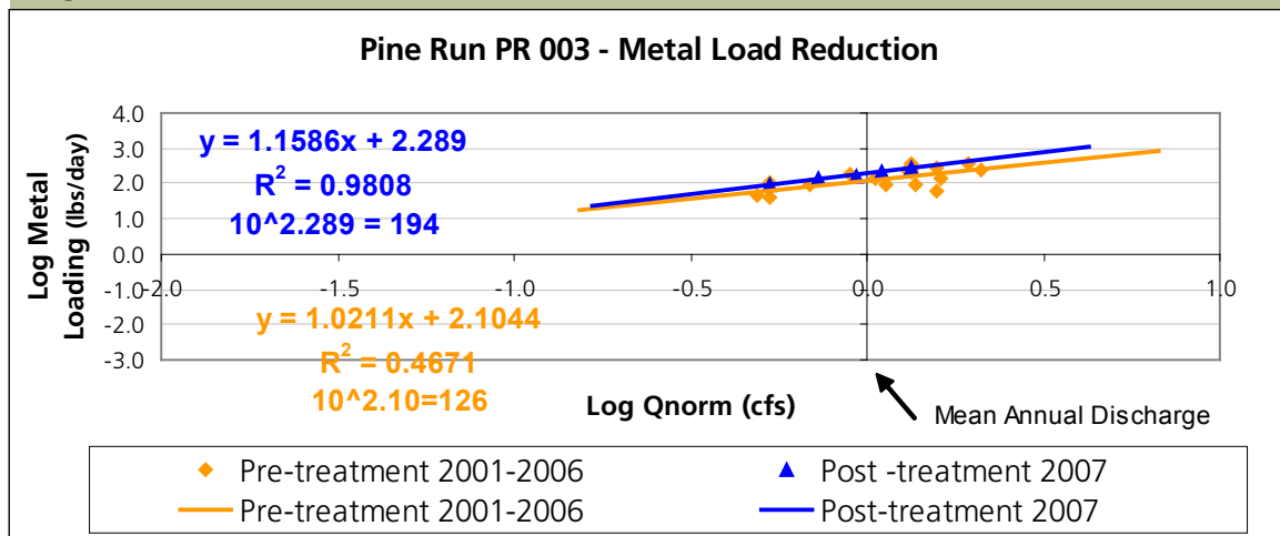
Figure 4. Metal Load Reduction
