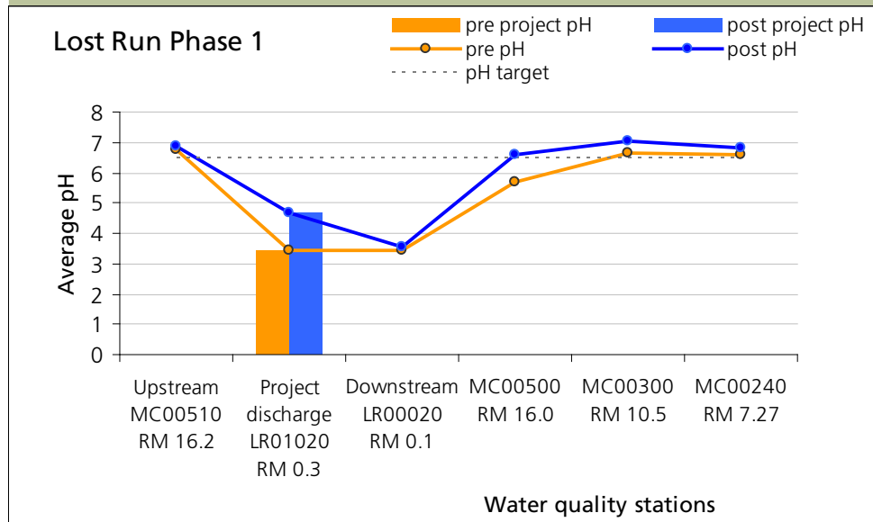
Figure 1. Pre and Post pH
